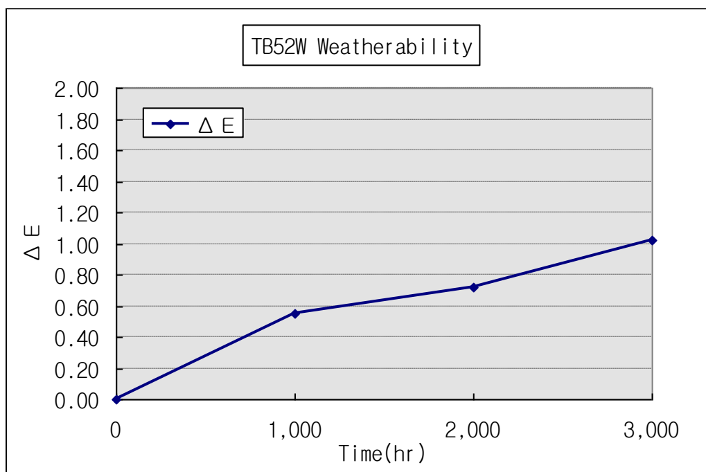
Figure. Weatherability of TB52W, Samsung's super weatherability and heat-resistant compound PP
